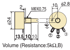
Volume (Resistance: 5kΩ, B)
